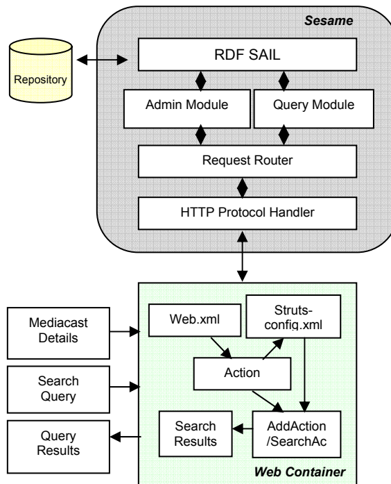
Figure 7: Publish/Subscribe architecture
