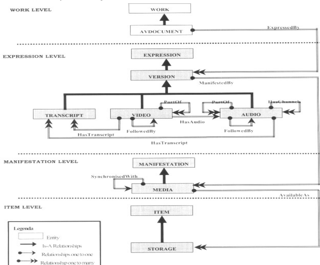
Figure 4. The ECHO metadata model
