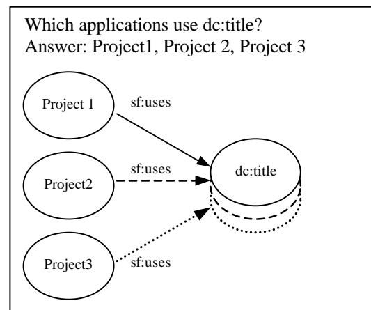
Figure 8. Joining statements as a basis for queries
